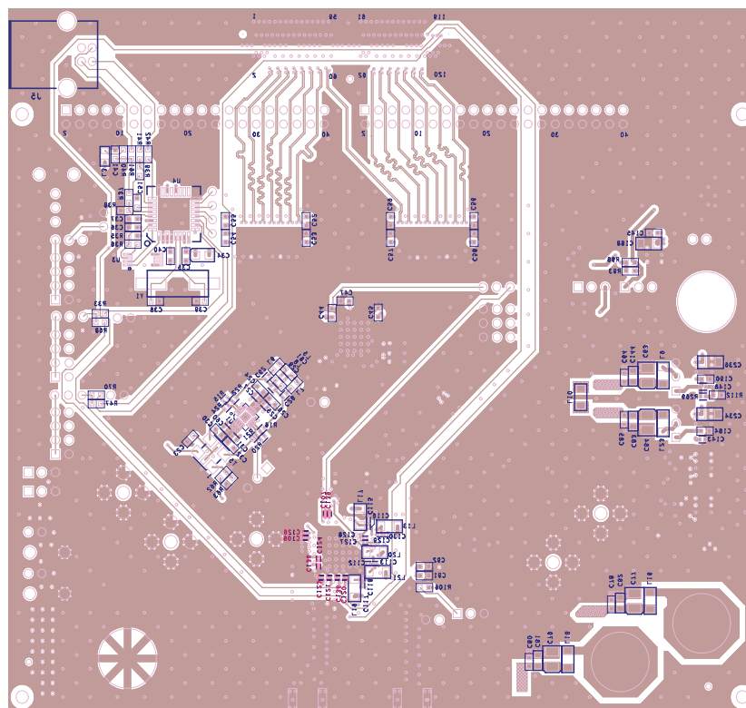
Figure 18. Bottom Side
