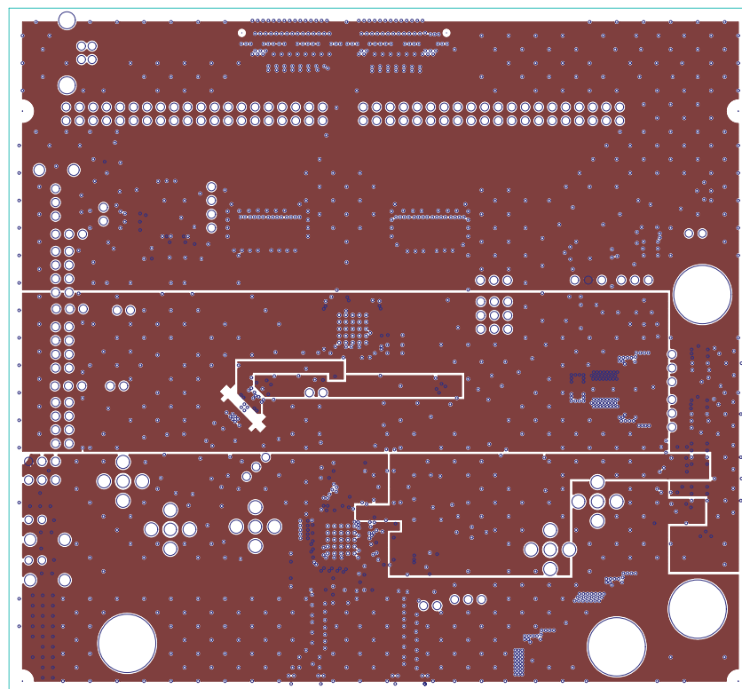
Figure 15. Power Plane 1
